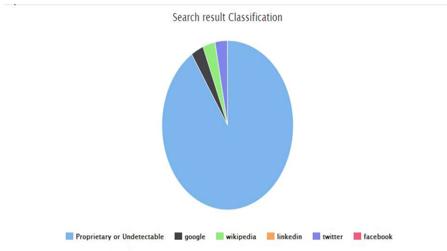
Fig 2.Domain classification
