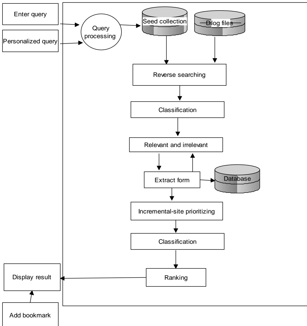
Fig.No.01) System architecture of smart crawler
